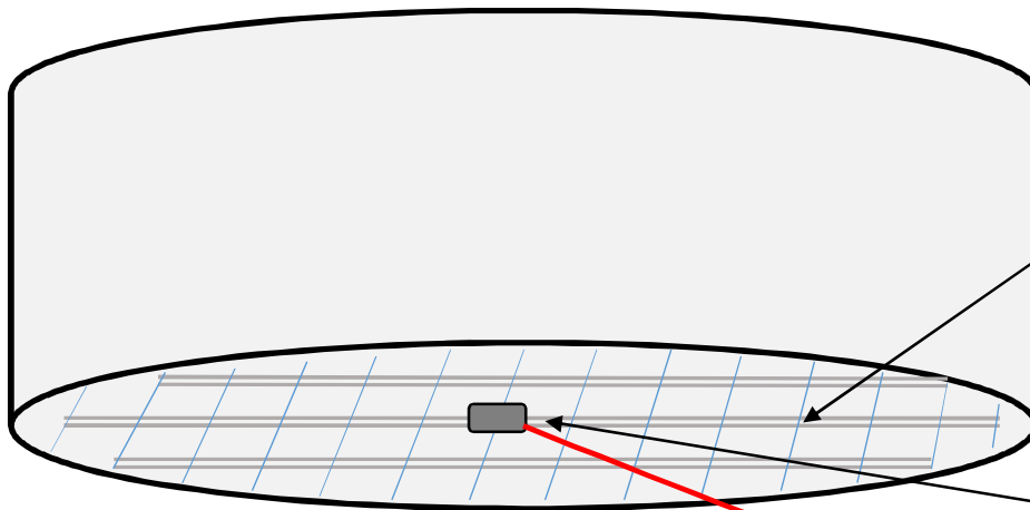
UNDERTANK GRID SYSTEM LAYOUT – MMO/Ti RIBBON / Ti CONDUCTOR BAR FOR EXTERNAL BASE PLATE PROTECTION.
